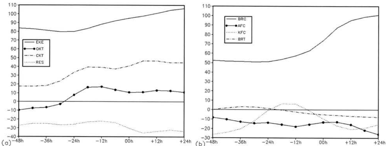
FIG. 16. As in Fig. 11, but for composite C.
