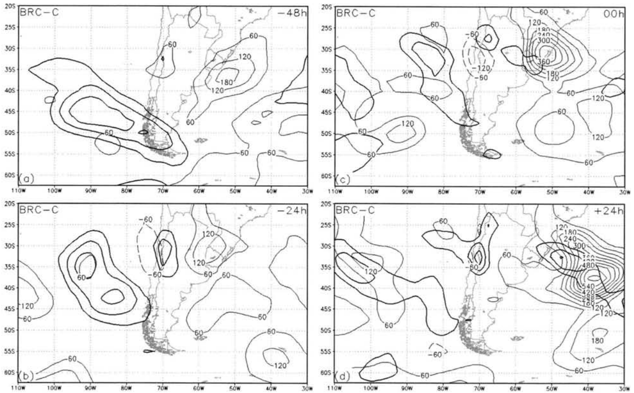
FIG. 13. As in Fig. 8, but for composite C.
