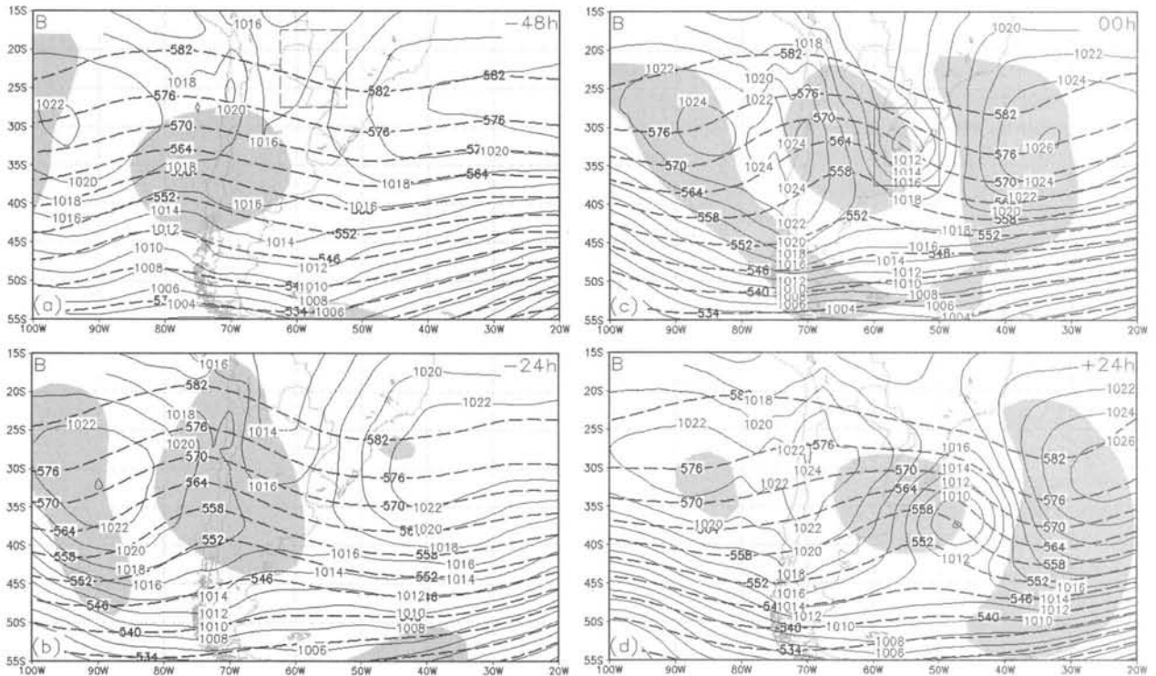
FIG. 3. (a)–(d) SLP [solid line, contour interval (CI) 2 hPa] and 500-hPa geopotential height (dashed line, CI 6 dam, shaded regions are statistically significant at level of 95%) of composite B. In (a), the box with dashed lines indicates the area where the spatial average of the heat and moisture flux shown in Fig. 5c were made. In (c), the box with solid lines shows the area where the spatial average of the variables shown in Figs. 5a,b and 6 were made. The time in the upper-right corners refers to the formation of the surface cyclone.
