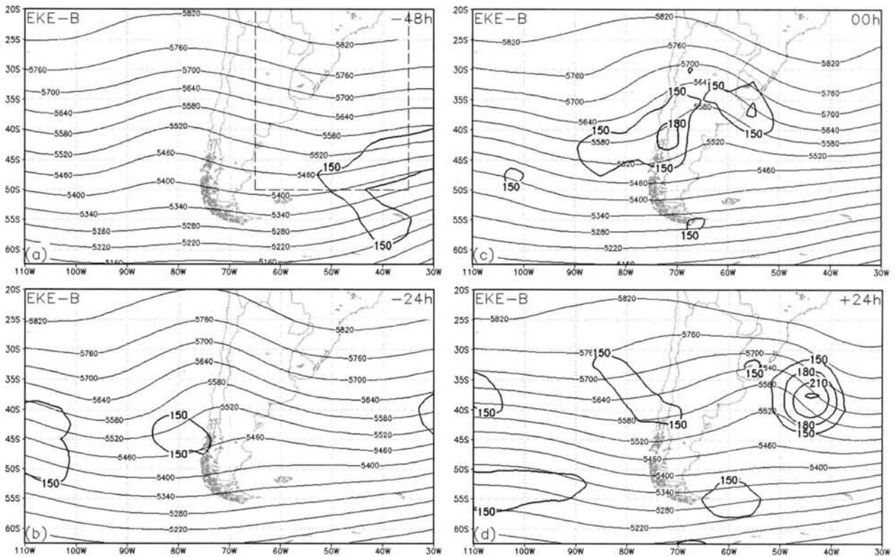
FIG. 7. (a)–(d) 500-hPa geopotential heights (CI 60 m) and vertically averaged EKE (CI 30 \text{m}^2 \text{s}^{-2} , values below 150 \text{m}^2 \text{s}^{-2} omitted) for composite B. In (a), the box with dashed lines represents the area where the volume average shown in Fig. 11 were made.
