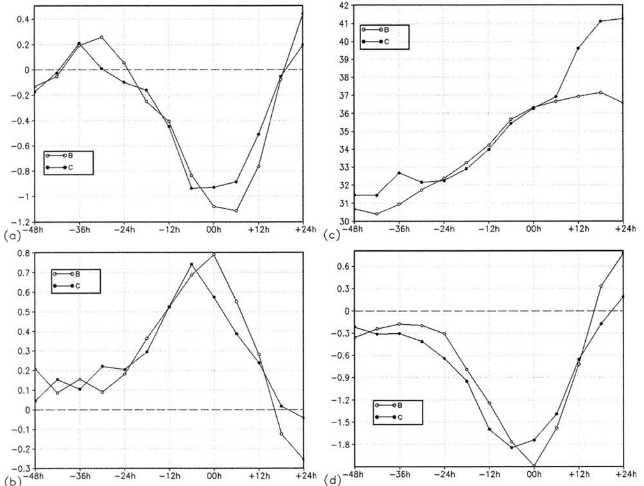
FIG. 6. As in Fig. 5, but for (a) relative vorticity advection ( \times 10^{-9} \text{ s}^{-2} ), (b) divergence ( \times 10^{-5} \text{ s}^{-1} ), (c) wind magnitude ( \text{m s}^{-1} ) at 300 hPa, and (d) vertical velocity ( \times 10 \text{ Pa s}^{-1} ) at 500 hPa.
