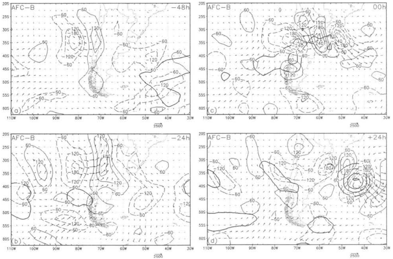
FIG. 9. As in Fig. 8, but for the AFC ( \text{CI } 60 \text{ m}^2 \text{ s}^{-2} \text{ day}^{-1} , zero omitted) term and ageostrophic flux vectors ( \text{m}^3 \text{ s}^{-3} ).
