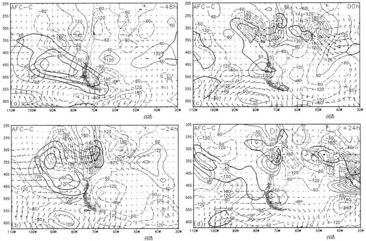
FIG. 14. As in Fig. 9, but for composite C.
