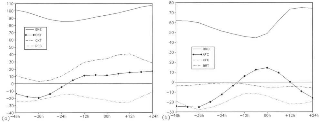
FIG. 11. Temporal evolution of volume-averaged EKE budget for composite B: (a) EKE (solid line), OKT (line with closed circle), CKT (dotted-dashed line), and RES (dotted line) evolution; (b) the evolution of KFC (dotted line), AFC (line with closed circle), BRC (solid line), and BRT (dotted-dashed line). Units are m^2 s^{-2} day^{-1} , except for the EKE unit which is m^2 s^{-2} .
