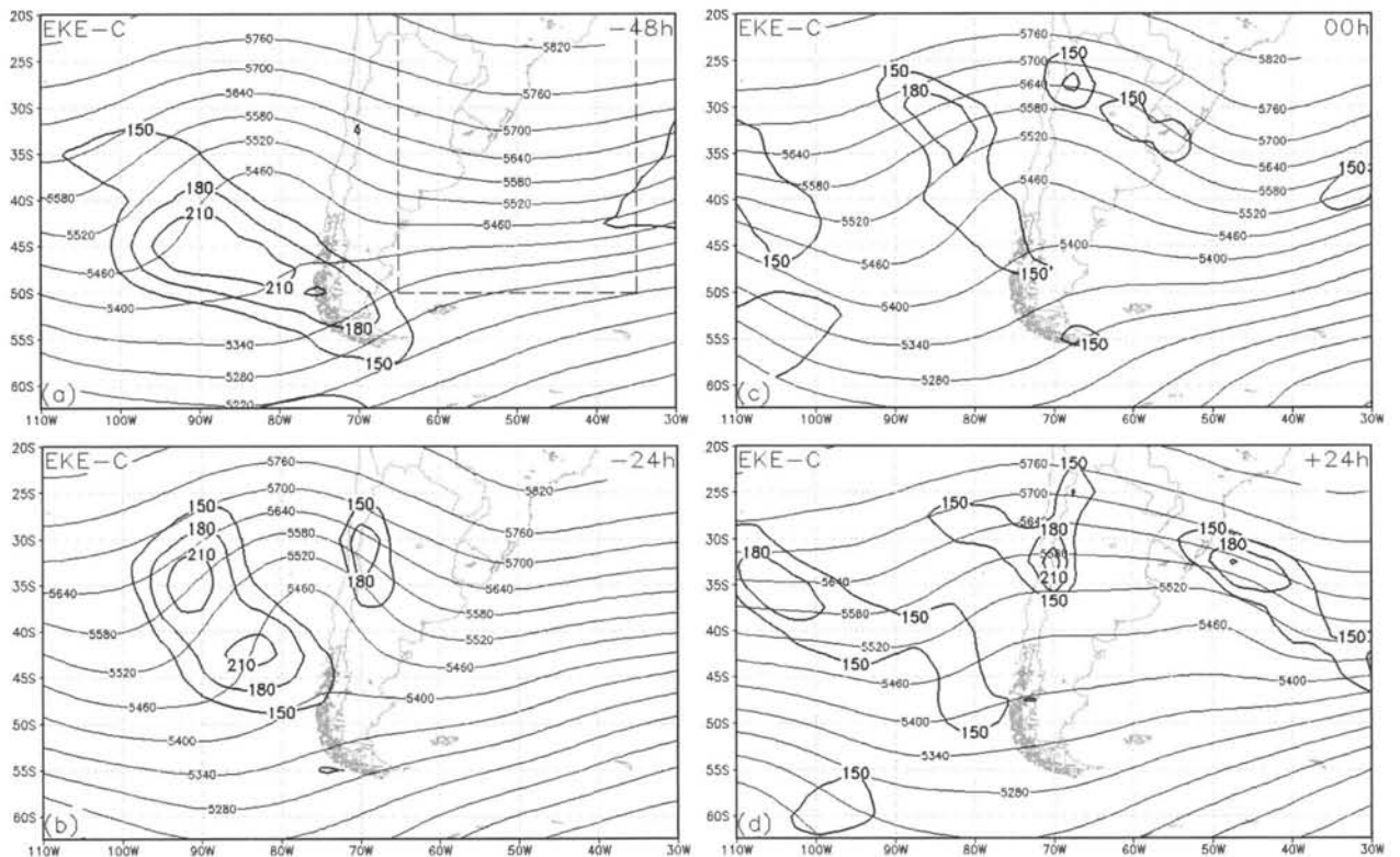
FIG. 12. As in Fig. 7, but for composite C.
