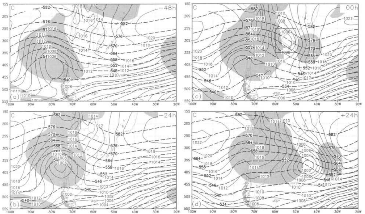
FIG. 4. As in Fig. 3, but for composite C.
