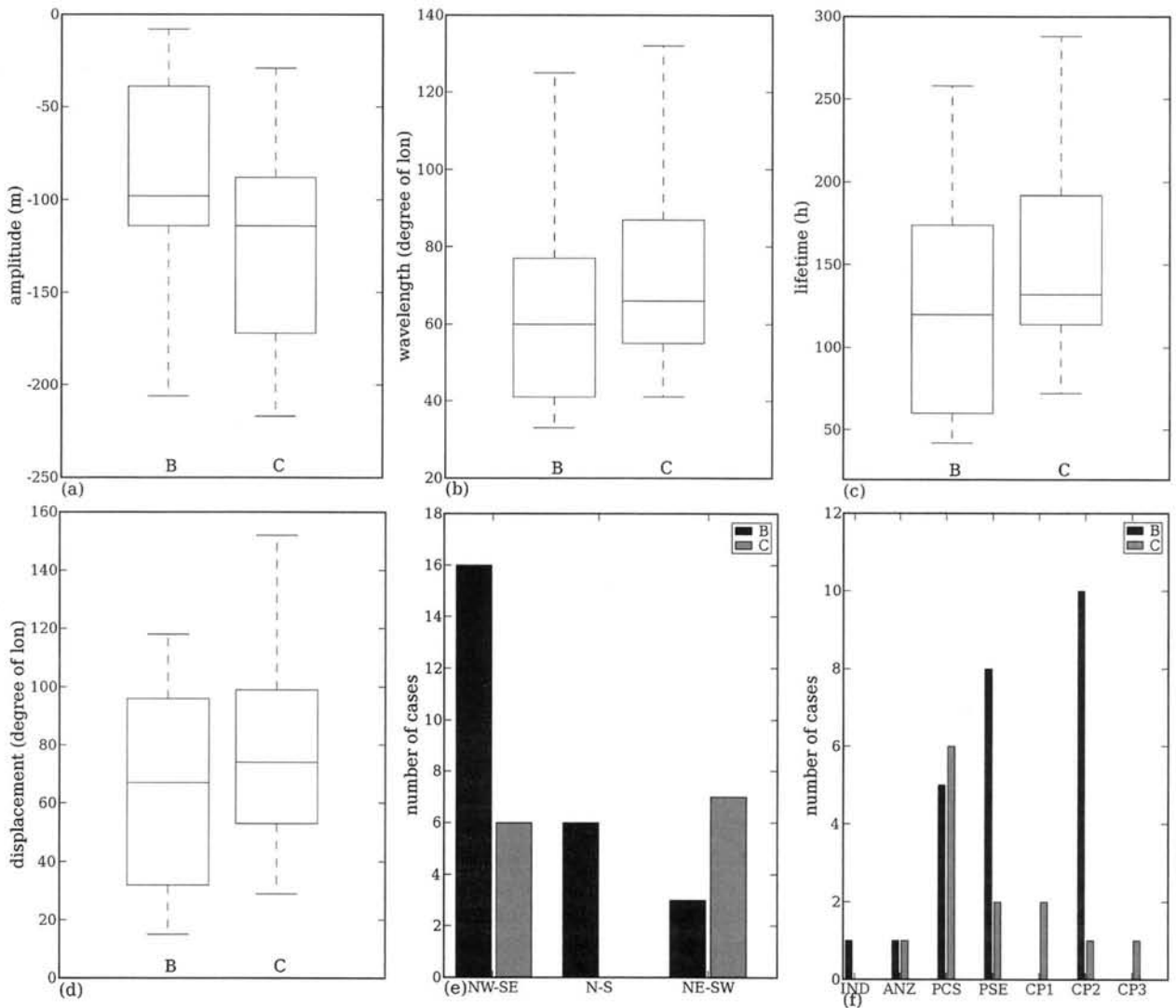
FIG. 1. Trough characteristics for the composites B and C: (a) amplitude (m), (b) wavelength ( ^{\circ} lon), (c) lifetime (h), (d) displacement ( ^{\circ} lon), (e) meridional tilting during cyclone formation time, and (f) genesis area as indicated in Fig. 2.
