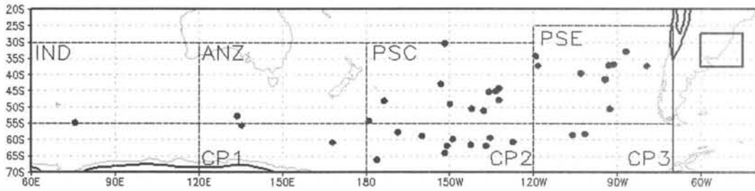
FIG. 2. Positions of trough formation for composites B and C. Genesis areas are the Indian Ocean (IND), Australia–New Zealand (ANZ), Pacific South Center (PSC), Pacific Southeast (PSE), and Circumpolar 1, 2, and 3 (CP1, CP2, and CP3), respectively. The box over the east coast of South America indicates the region where the surface cyclones must be stationed to be considered in the composites. Topography (km, thick isoline, label omitted) over South America corresponds to 1.5, 3, and 4.5 km.
