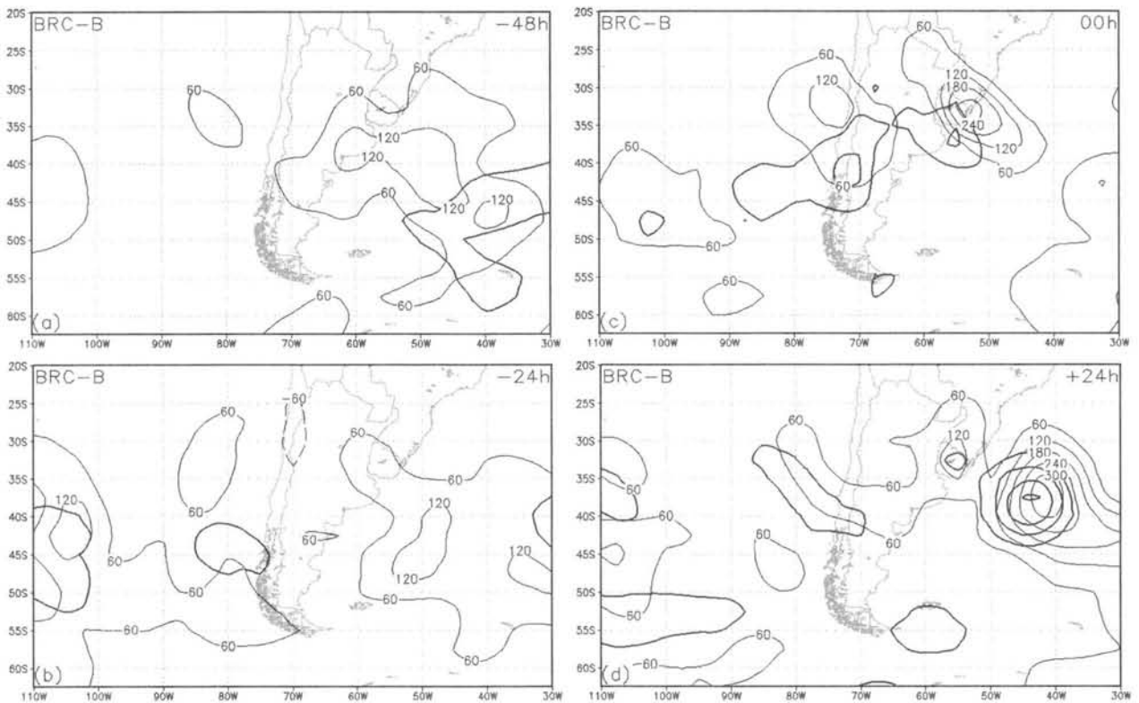
FIG. 8. BRC term ( \text{CI } 60 \text{ m}^2 \text{ s}^{-2} \text{ day}^{-1} , zero omitted) and vertically averaged EKE (thick lines, label omitted) for composite B at (a) -48 , (b) -24 , (c) 0 , and (d) +24 h.
